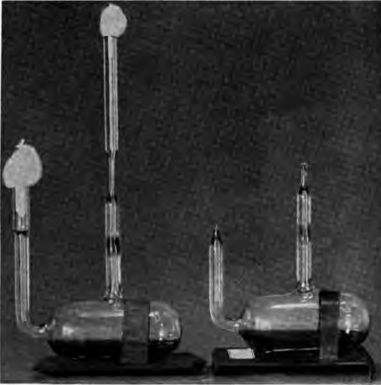
Fig. 7.—Fermentation bulb (after Rogers, Clark, and Davis). The side arm serves for introduction of the medium and inoculation; it is then sealed off. The other tube is used for exhaustion of the air (by the Boltwood mercury pump) and is then sealed as shown.
